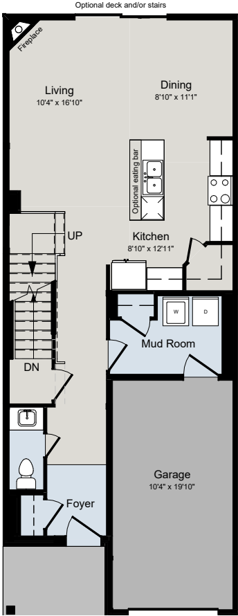
MAIN FLOOR
